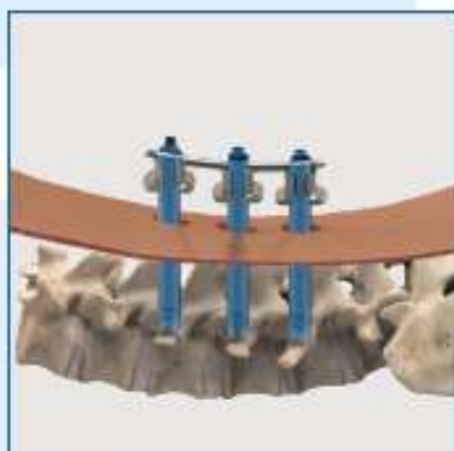
5. Rod Measurement
